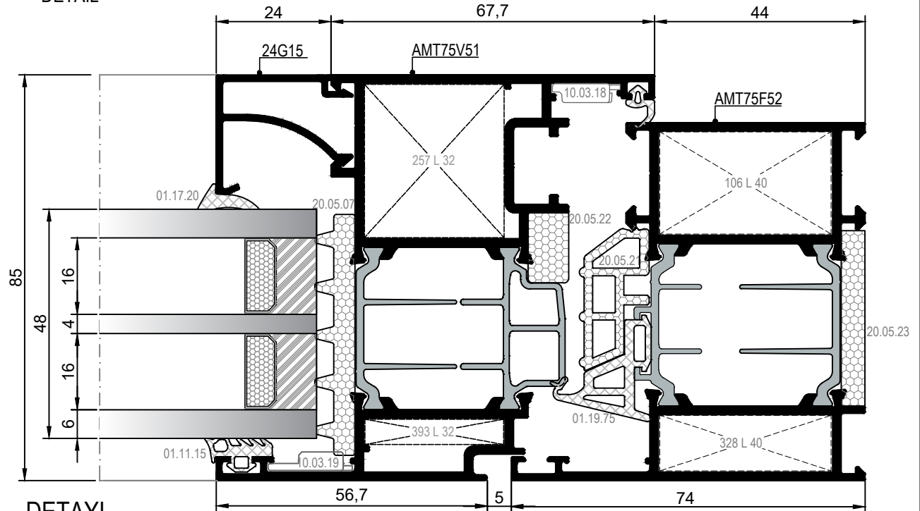
4A DETAYI DETAIL
