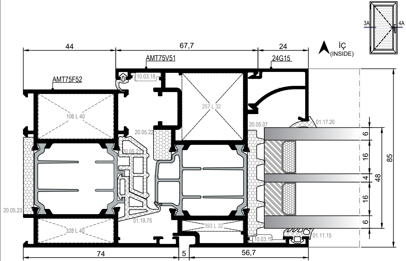
3A DETAYI DETAIL
