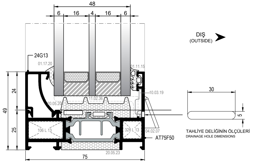
② DETAYI DETAIL
