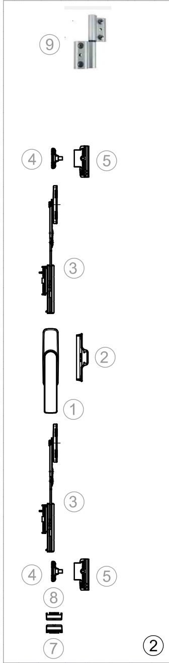
Fapim Out Casement Matrix W/Out Corner (2 Mechanism)
