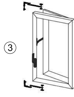
Fapim Out Casement Matris W/Corner (1 Mechanism)
