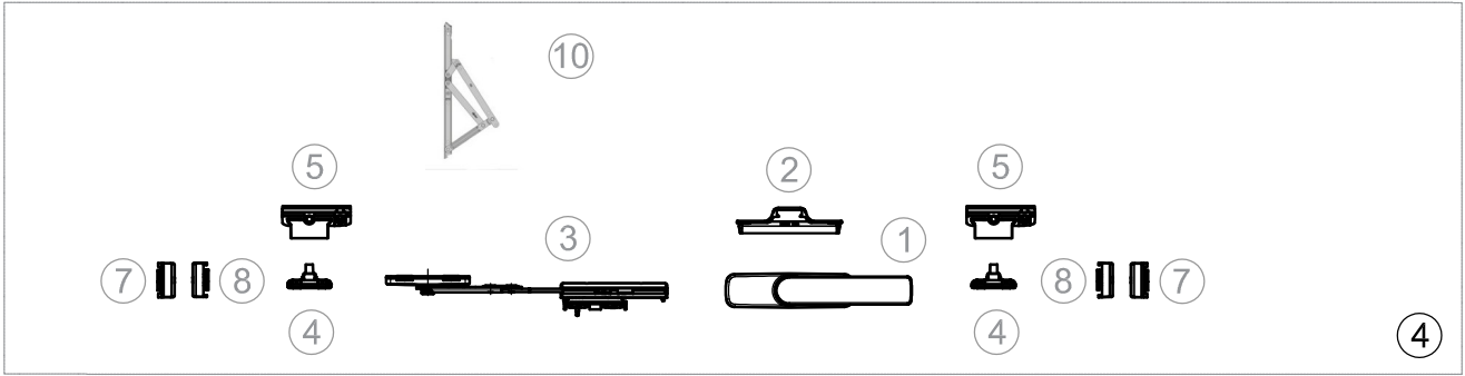
Fapim Out Awning Matrix W/Out Corner (1 Mechanism)
