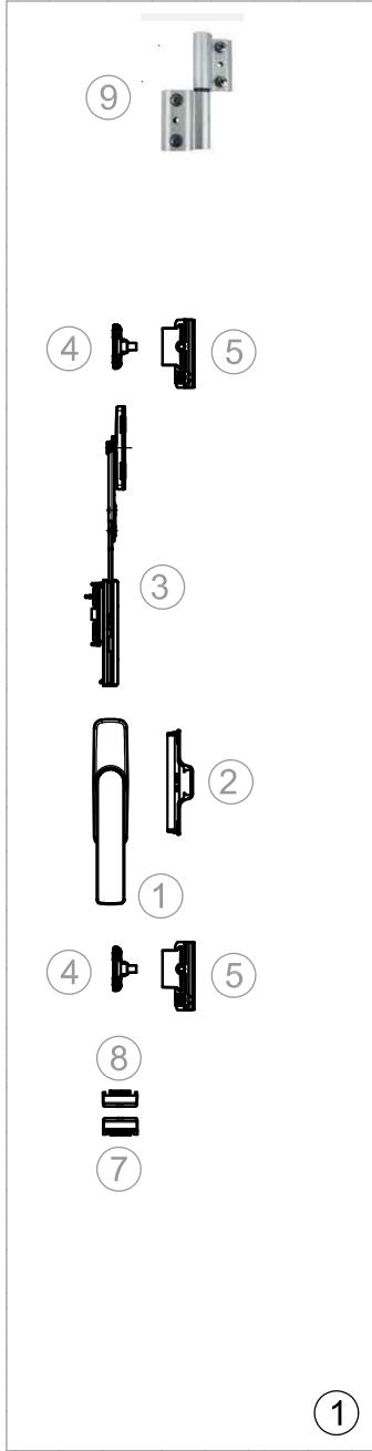
Fapim Out Casement Matrix W/Out Corner (1 Mechanism)
