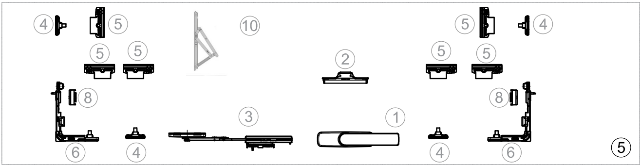
Fapim Out Awning Matrix W/Corner (1 Mechanism)
