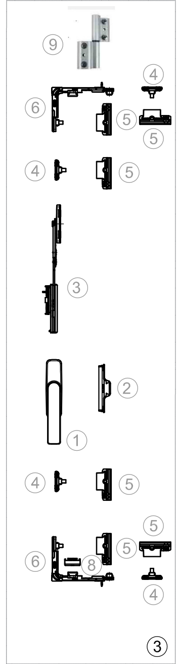
Fapim Out Casement Matrix W/Corner (1 Mechanism)
