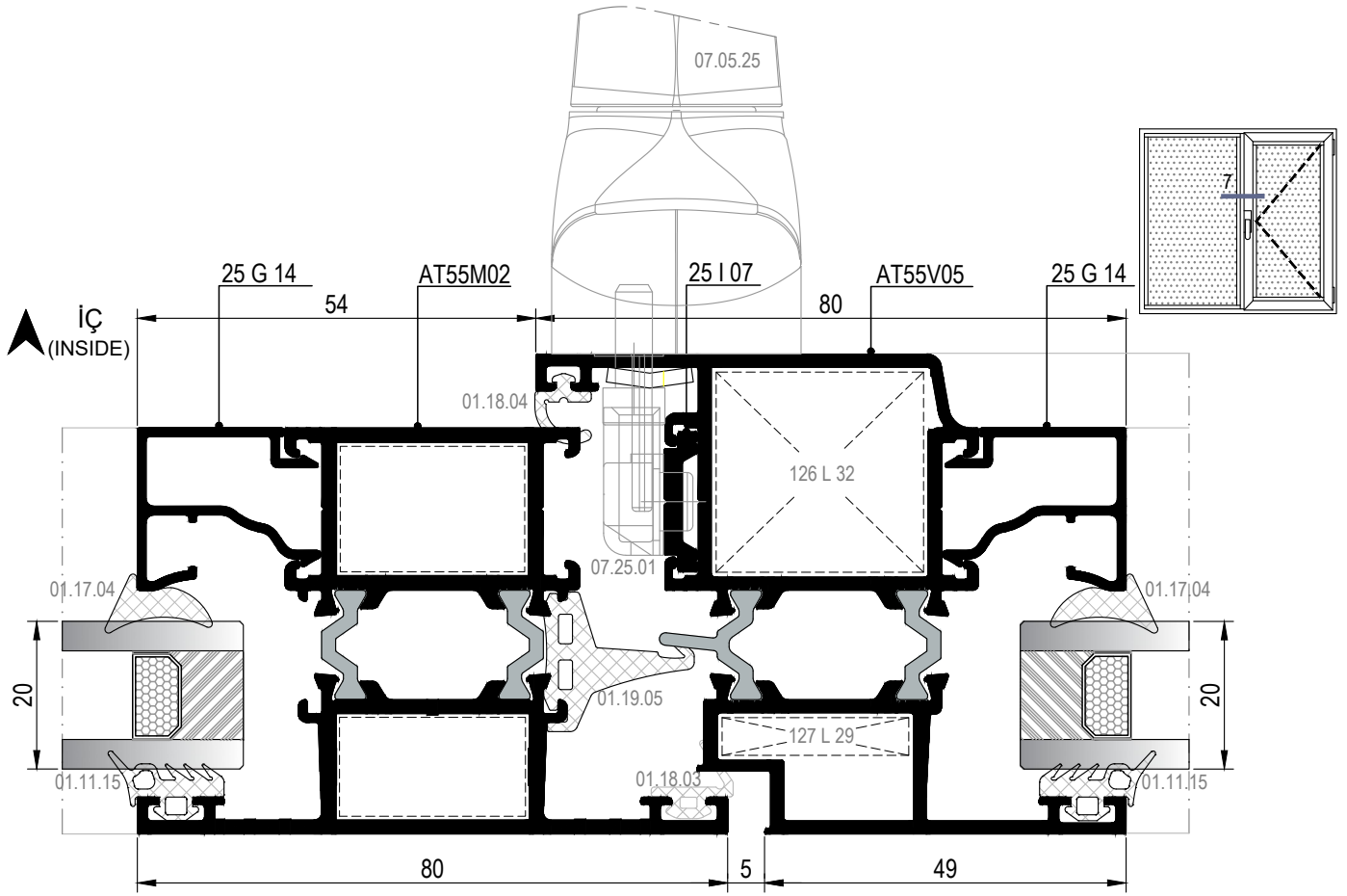
7 DETAYI DETAIL
