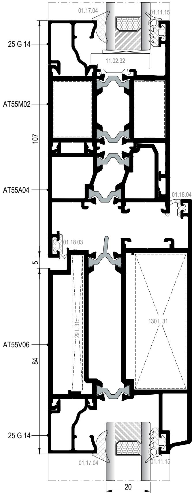
35 DETAYI DETAIL
