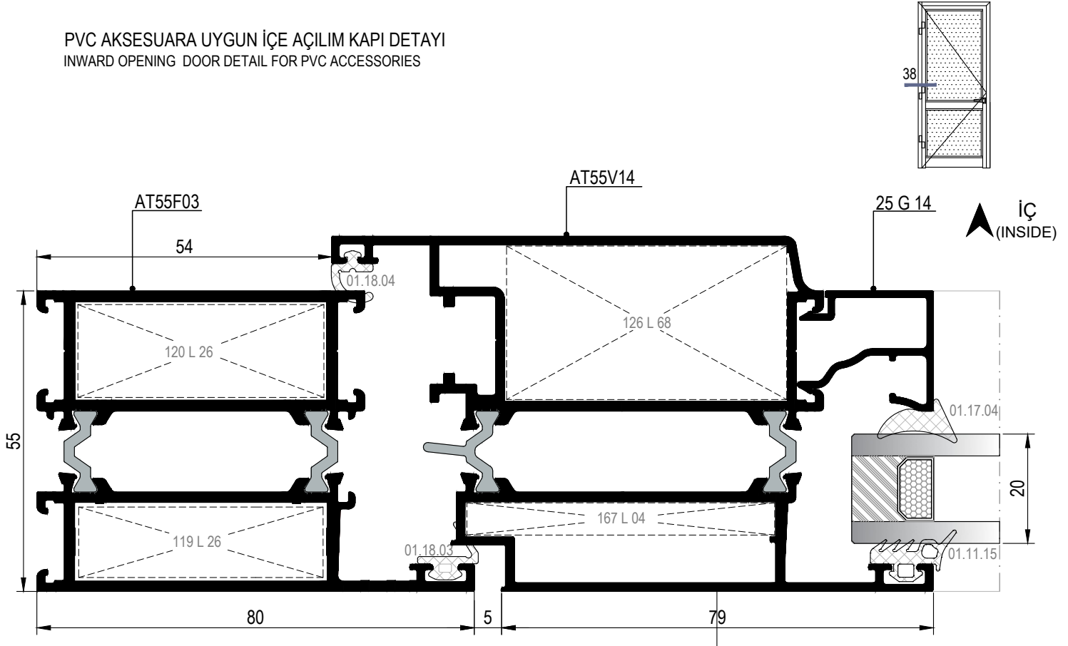
38 DETAYI DETAIL
