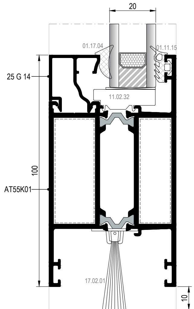
36 DETAYI DETAIL
