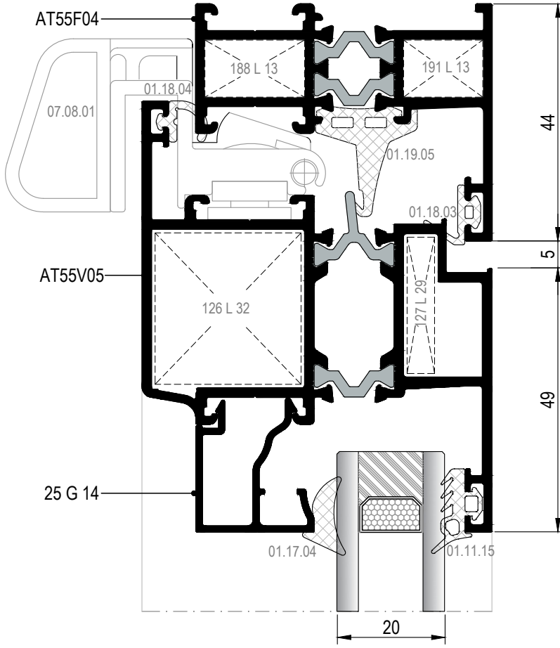
5 DETAYI DETAIL
