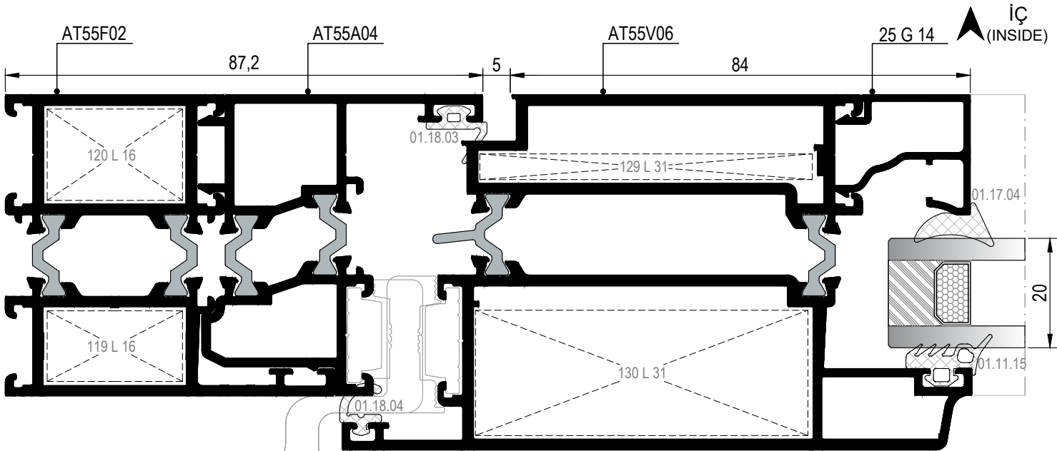
34 DETAYI DETAIL
