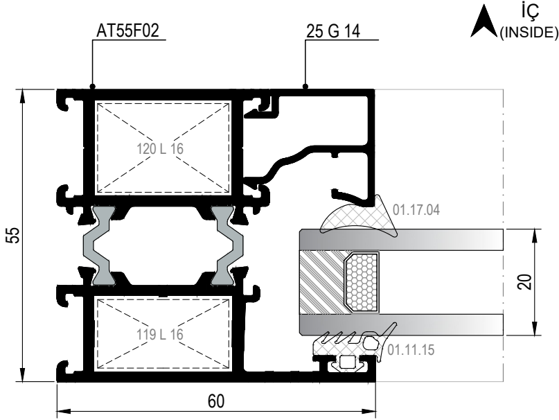
33 DETAYI DETAIL
