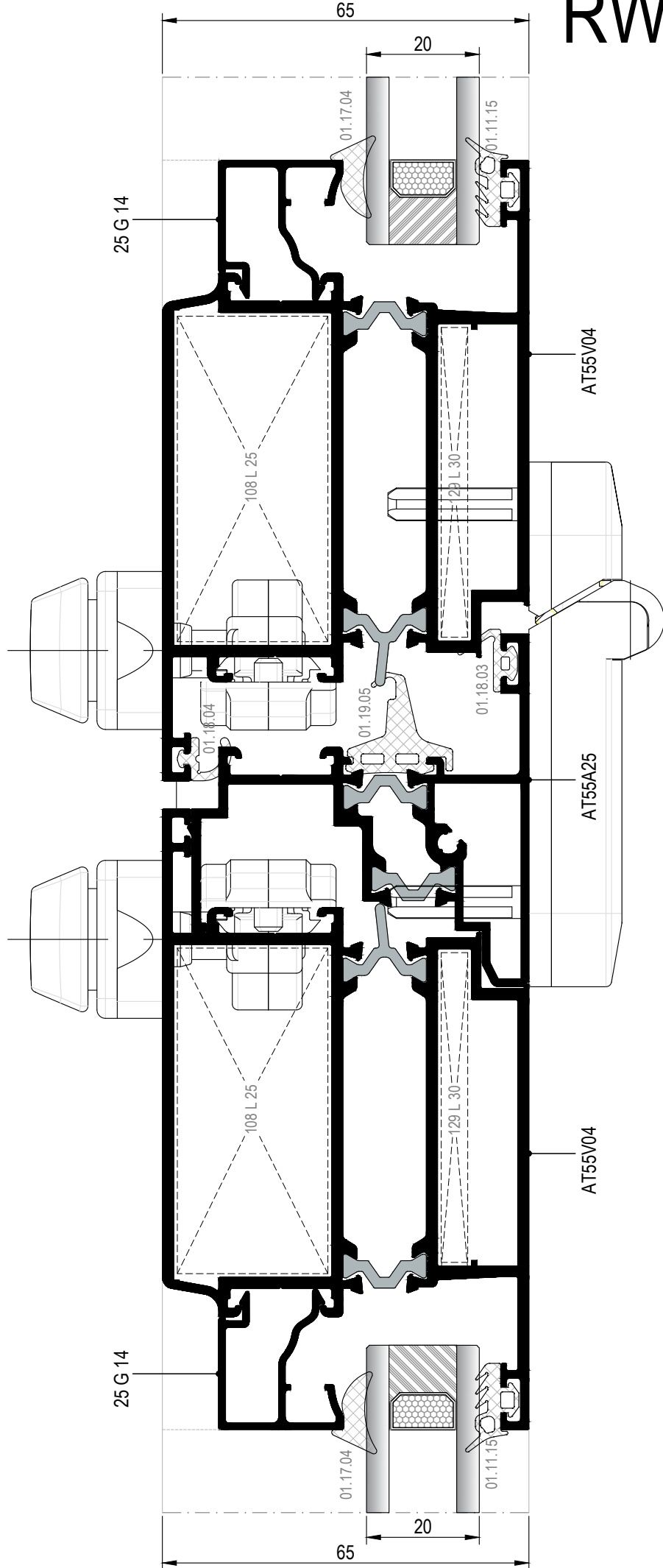
KATLANIR KAPI DETAYI FOLDING DOOR DETAILS
