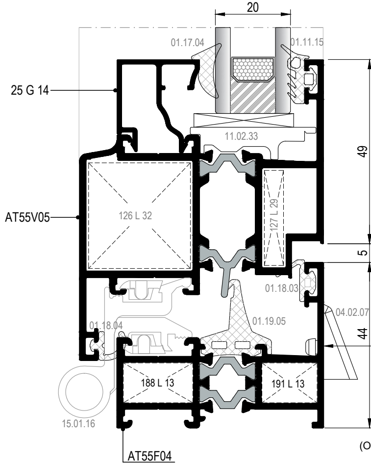
6 DETAYI DETAIL
