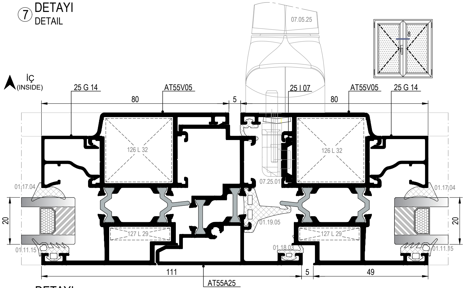
8 DETAYI DETAIL
